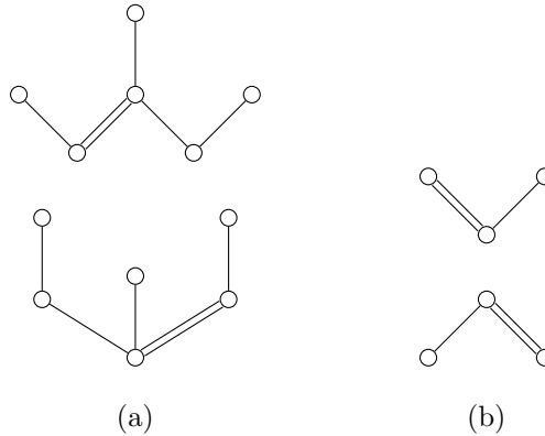
FIGURE 4.1. Pairs of labeled trees with the same K_{(P,\omega)}
