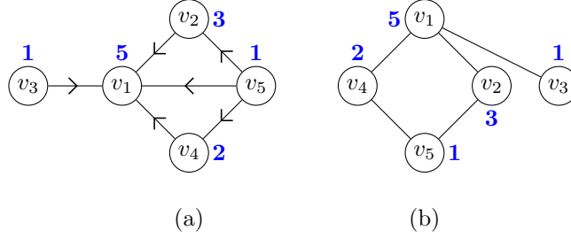
FIGURE 2.1. Converting from a proper coloring of a digraph to a strict P -partition. The numbers next to each node correspond to a coloring in the digraph on the left and the corresponding (P, \omega) -partition of the labeled poset on the right.
