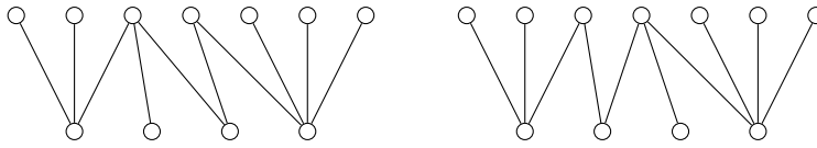
FIGURE 3.1. Two trees of rank one with the same degree sequences but different K_P
