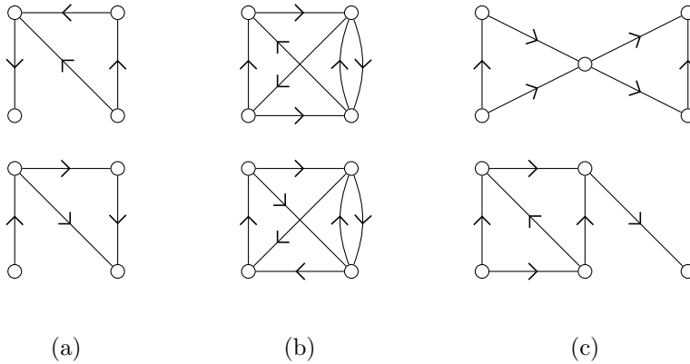
FIGURE 1.1. Pairs of digraphs with equal chromatic quasisymmetric functions
