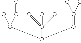
FIGURE 4.2. Example of a fair tree of size 13.
