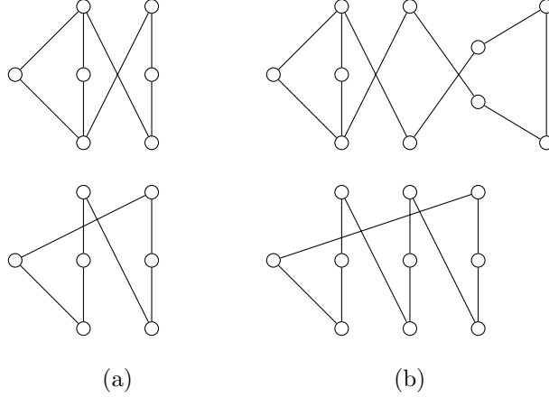
FIGURE 2.3. Pairs of posets with equal P -partition enumerators
