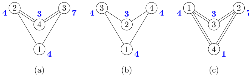
FIGURE 2.2. Examples of (P, \omega) -partitions
