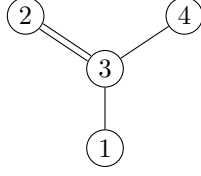
FIGURE 2.5. The labeled poset of Example 2.6
