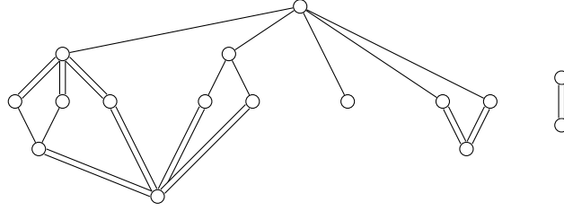
FIGURE 4.3. Example of an element of \mathcal{C} of size 16.
