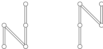
FIGURE 2.4. The strict P -partition enumerators of these two posets have the same F -support
